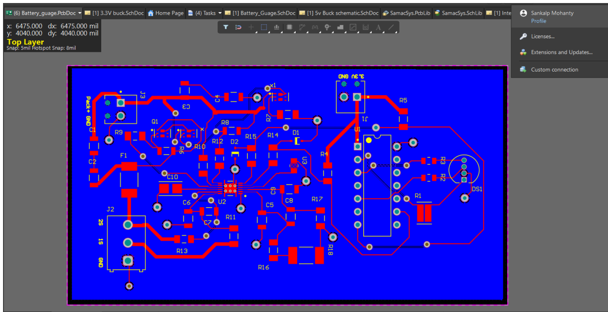
Layout of Fuel Guage Battery Monitoring Board
